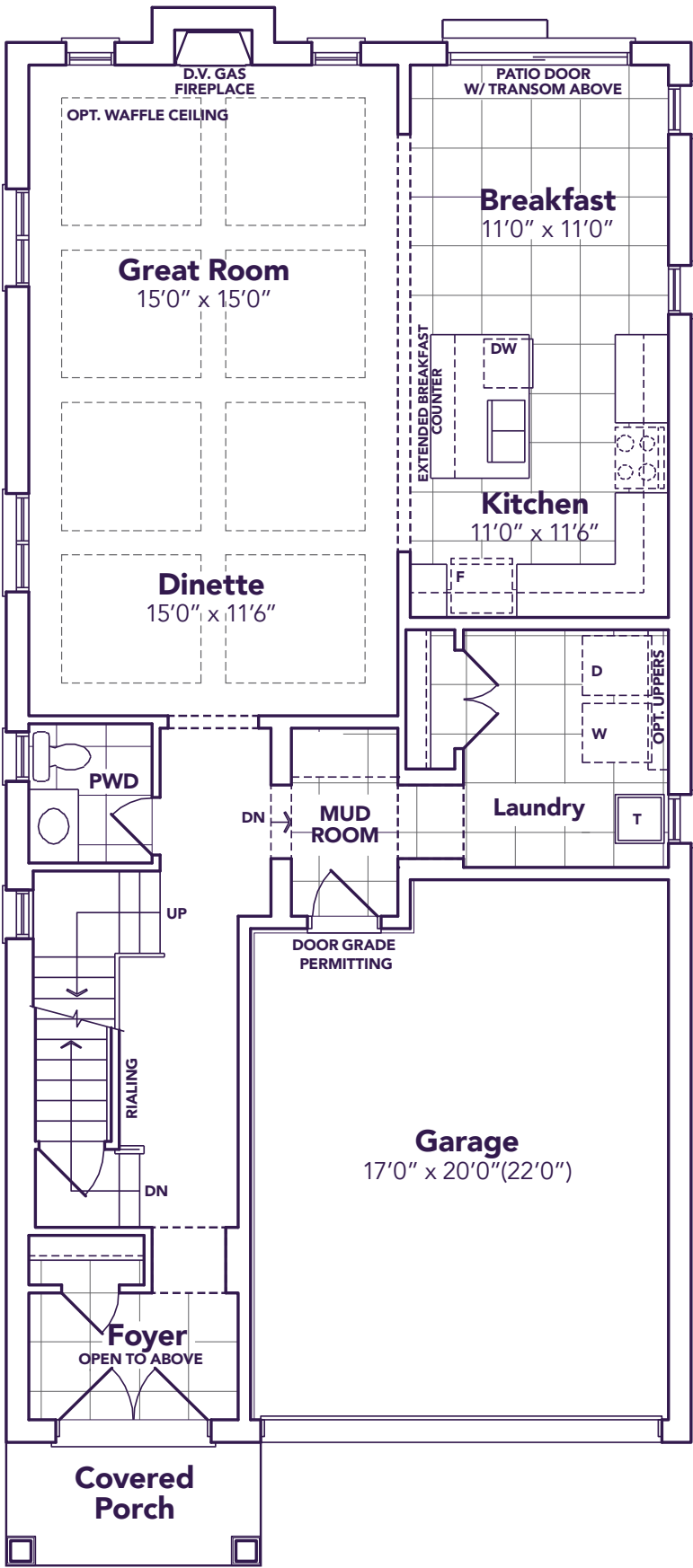
ELEVATION A MAIN FLOOR
