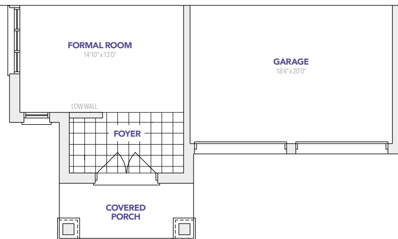
B PARTIAL MAIN FLOOR
