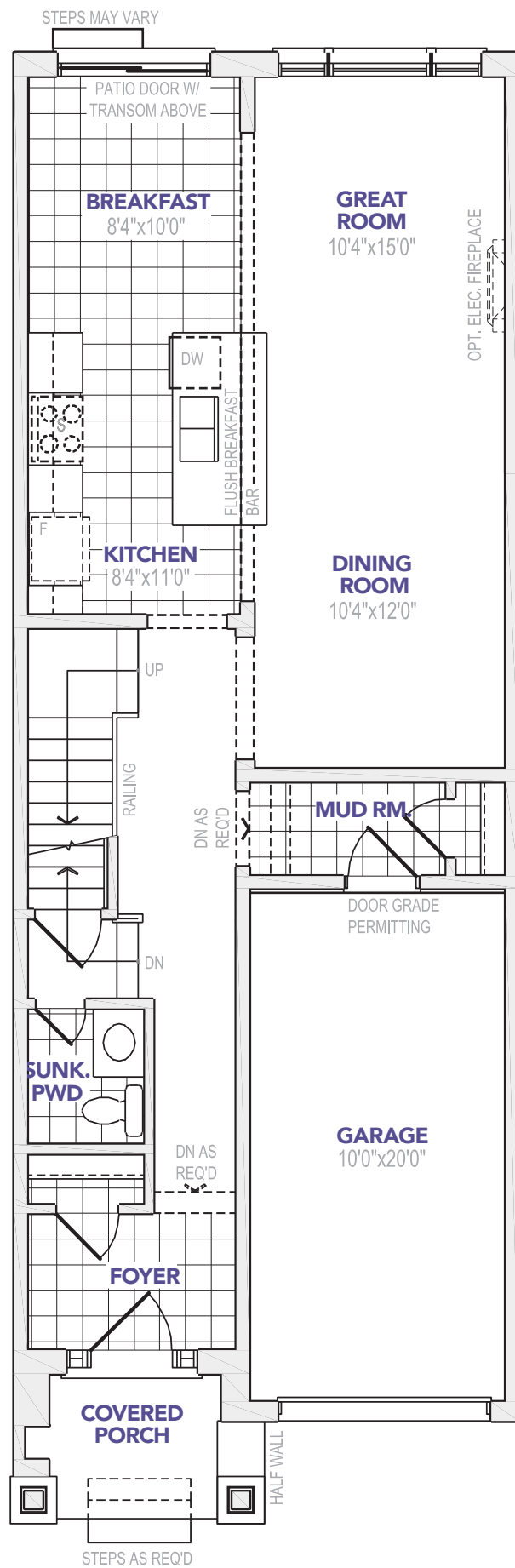
A MAIN FLOOR
