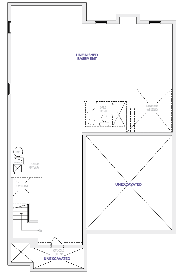
A BASEMENT
