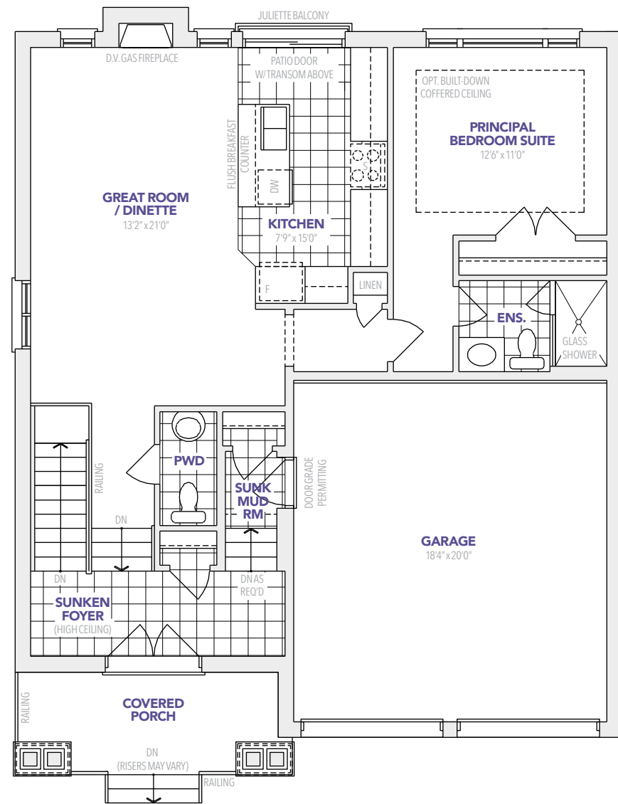
A MAIN FLOOR
