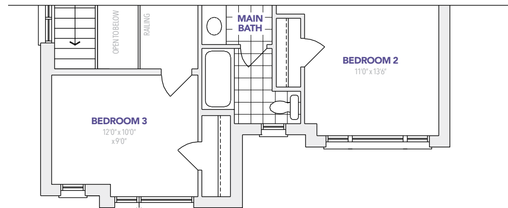
B PARTIAL SECOND FLOOR
