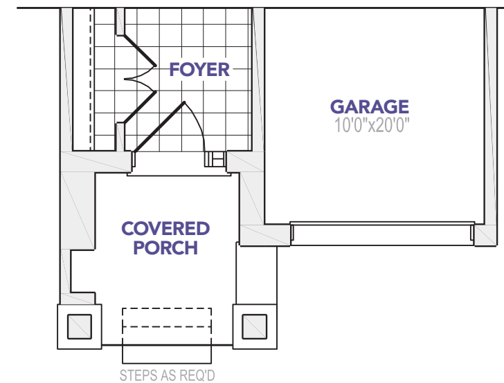
B PARTIAL MAIN FLOOR
