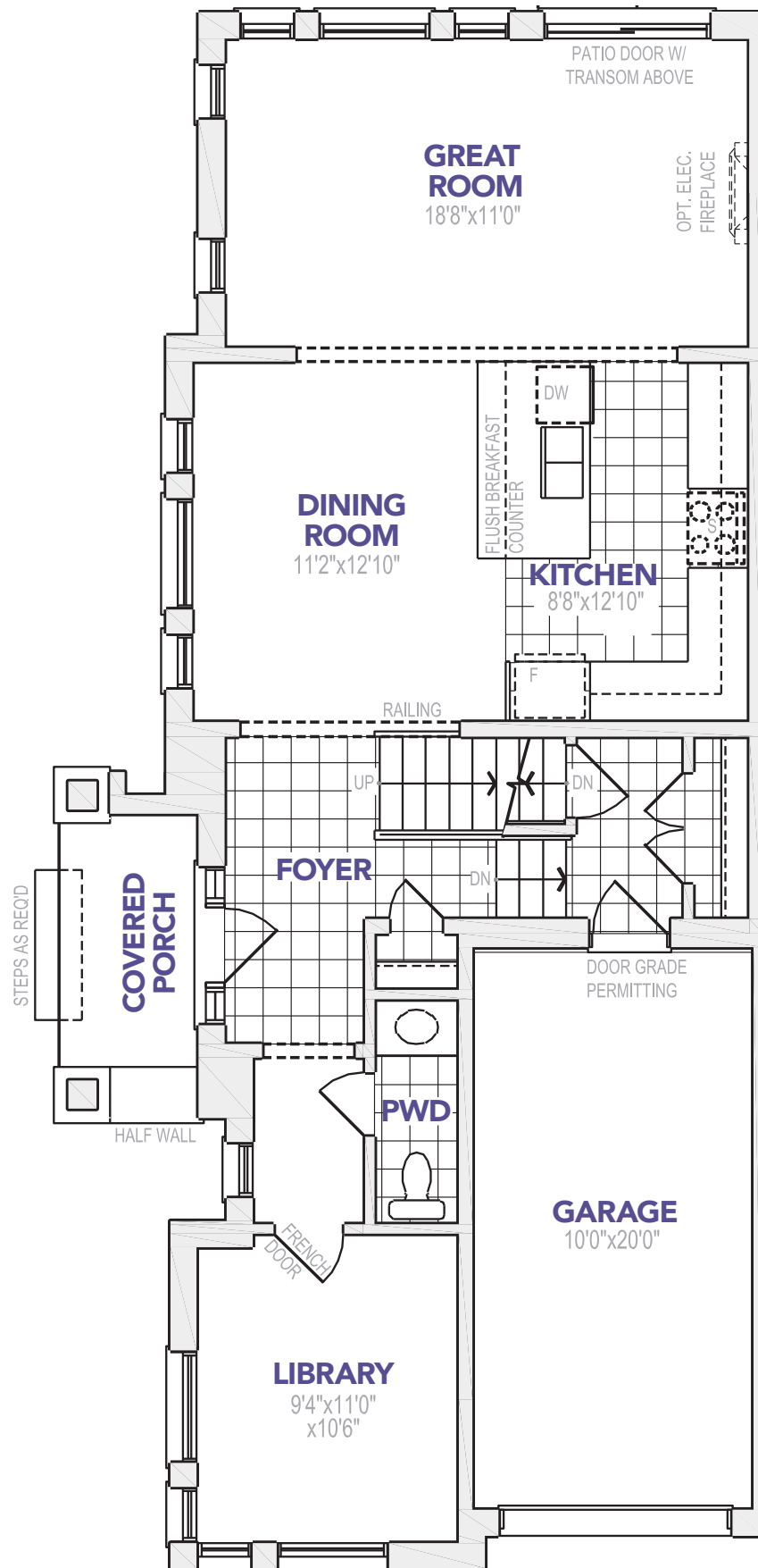
B MAIN FLOOR
