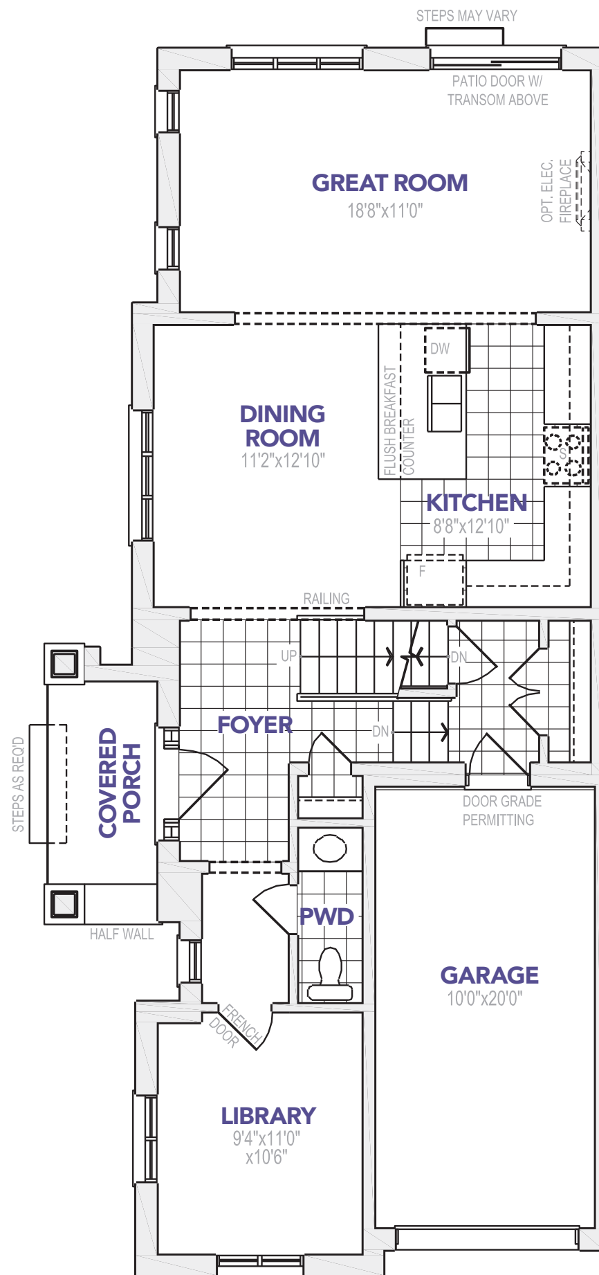
A MAIN FLOOR
