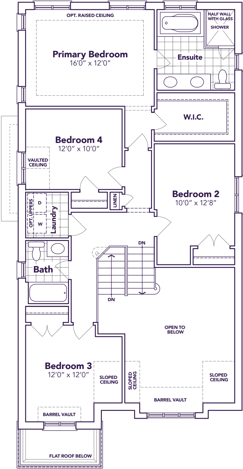
ELEVATION B SECOND FLOOR
