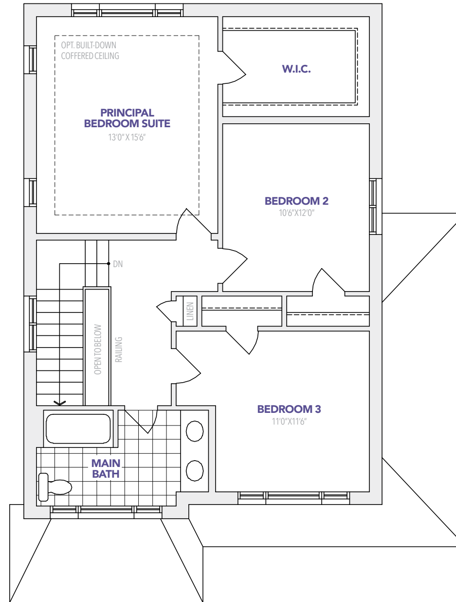
A SECOND FLOOR
